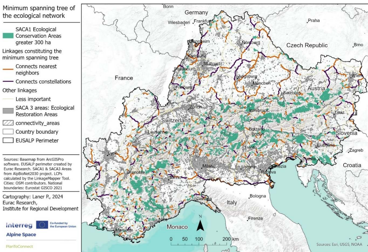
Figure 8: Minimum spanning tree
